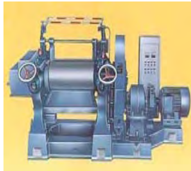
UXK-450 RUBBER MIXING MILL ROLLER
